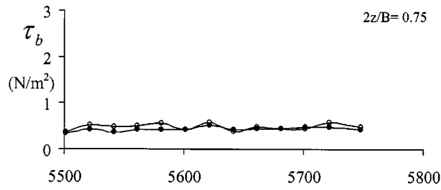
Fig. 12. Distribution of local boundary shear stresses between two consecutive nozzles
